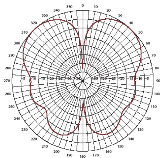
485 MHz Elevation Pattern
