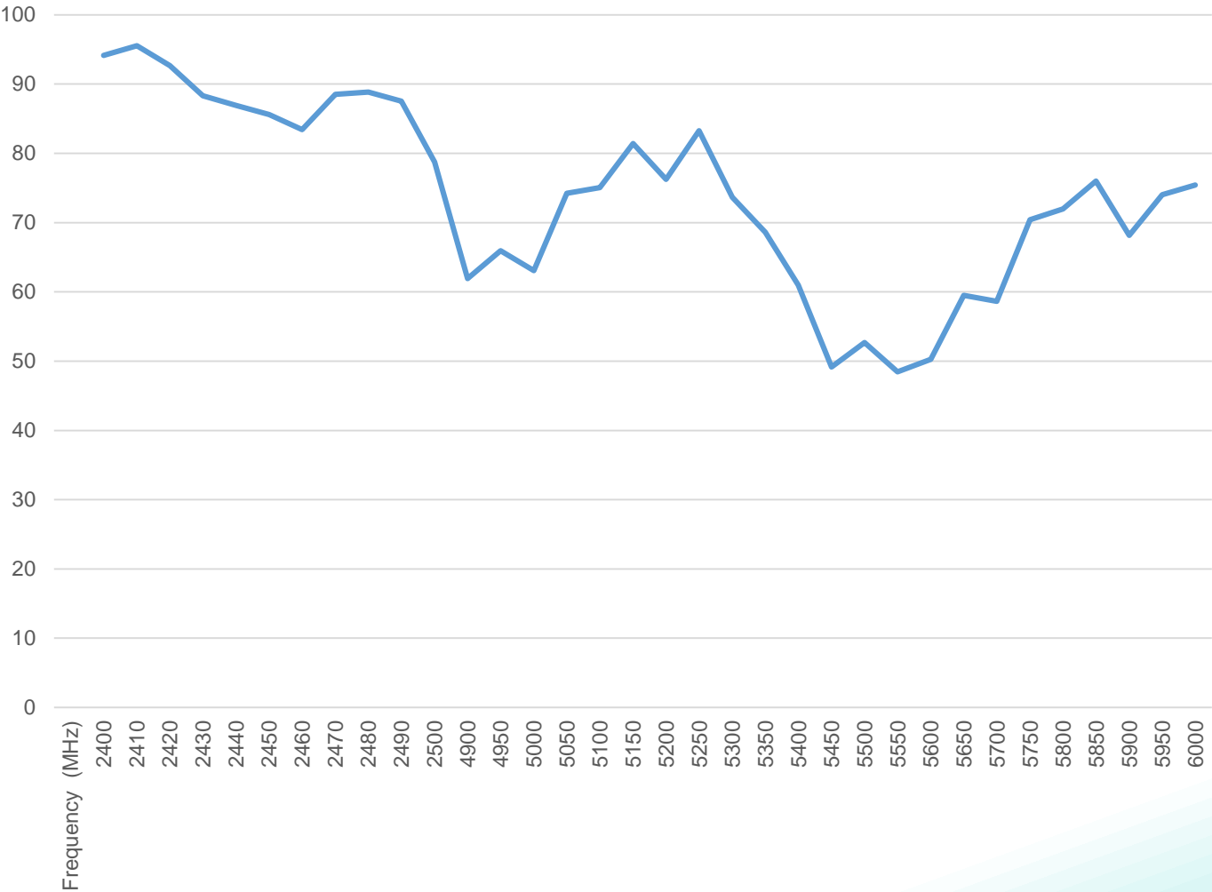
ICEFINWDMN Efficiency (%)
